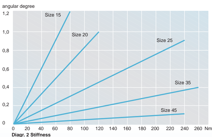
Diagr. 2 Stiffness
